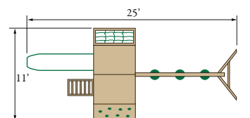
7C: Cliff Climb (tire swing included) with tarp roof, wonder wave slide, three-position 9' A-frame set, two swings, and plastic glider.
